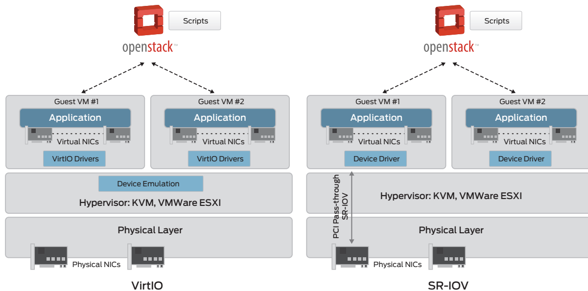
Figure 1: The vMX architecture for VirtIO and SR-IOV.
